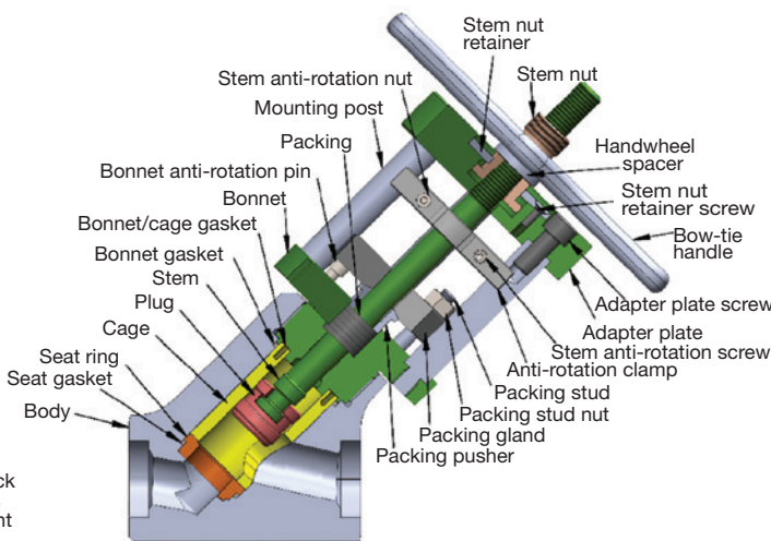
2. MPS-YPG globe valve eliminates costly and time-consuming repairs
